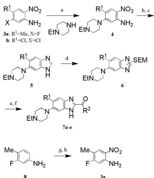
Scheme 1. Reagents and conditions: (a) K 2 CO 3 , DMSO, 120 °C; (b) Fe, NH 4 Cl, THF–MeOH–H 2 O, reflux; (c) HCO 2 H, 100 °C; (d) SEMCl, NaH, THF, 55–74% (4steps); (e) R–CO 2 Et, LTMP, THF, –78 °C, 46–55%; (f) TBAF, THF, reflux, 57–93%; (g) KNO 3 , TFAA, rt; (h) K 2 CO 3 , MeOH–H 2 O, rt, 66% (2 steps).
