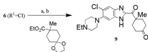
Scheme 2. Reagents and conditions: (a) LTMP, THF, –78 °C, 56%; (b) TFA–H 2 O (10:1), rt, 99%.
